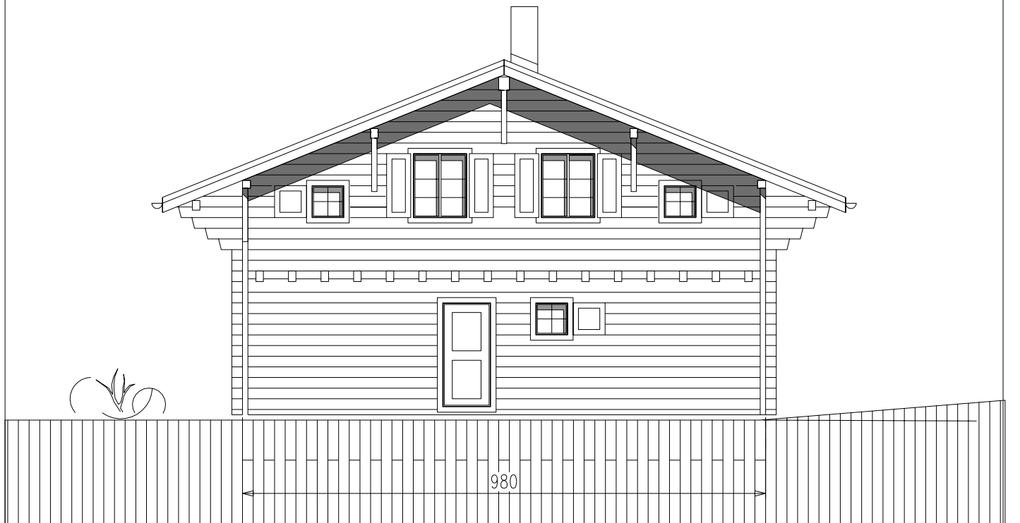
Facade Sud
