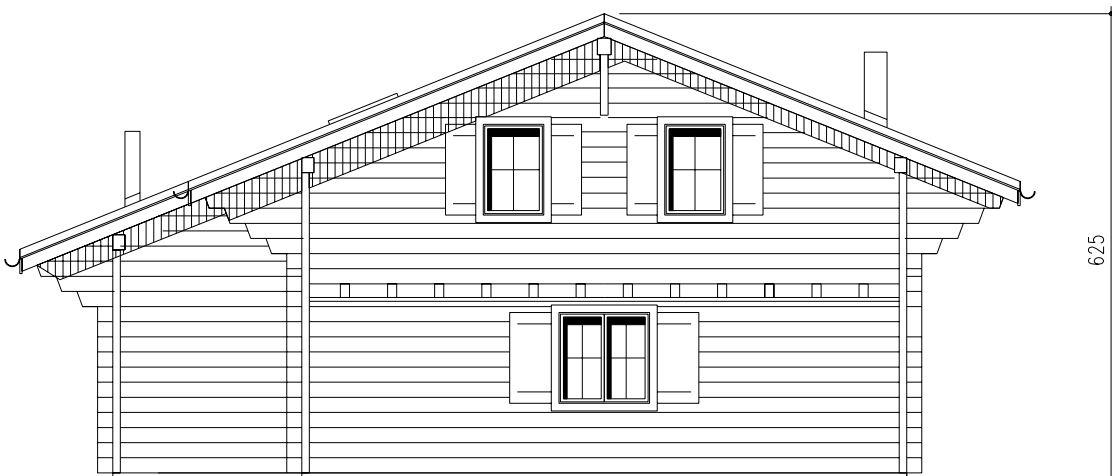
Facade SUD
